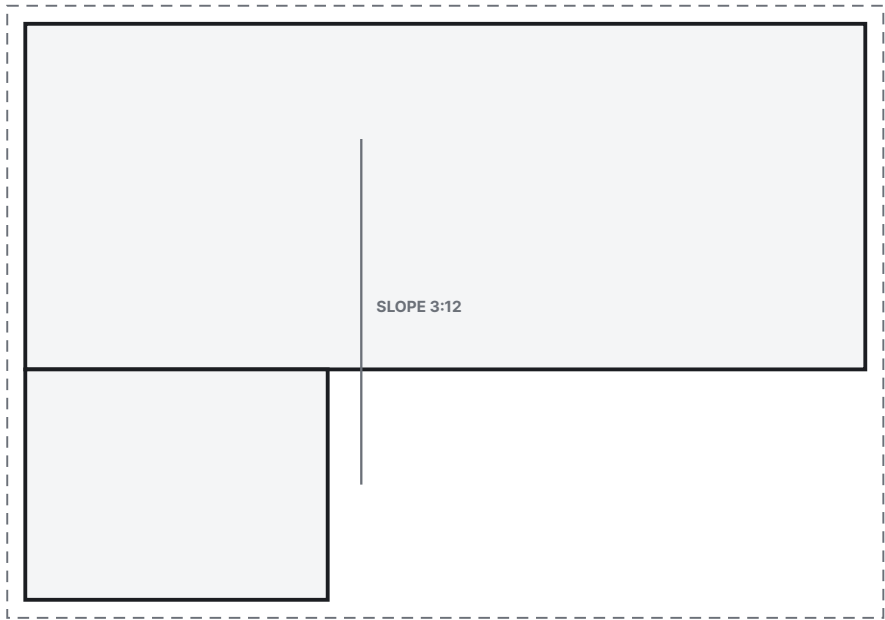
PSG6-300 roof panels spanning 32' max
